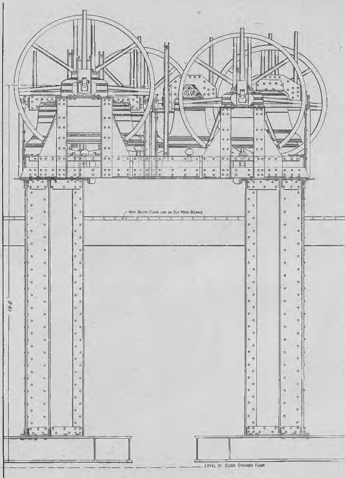
Vertical Cantilever Bell Frame for St. Michael's Church, Bray-on-Thames (Patent No. 14148.) (Tenor 26 cwt., Note D.)
